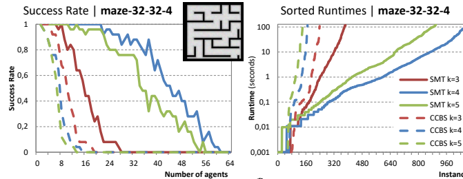
Fig. 4. Comparison of SMT-CBS ^{\mathcal{R}} and CCBS on maze-32-32-4.
