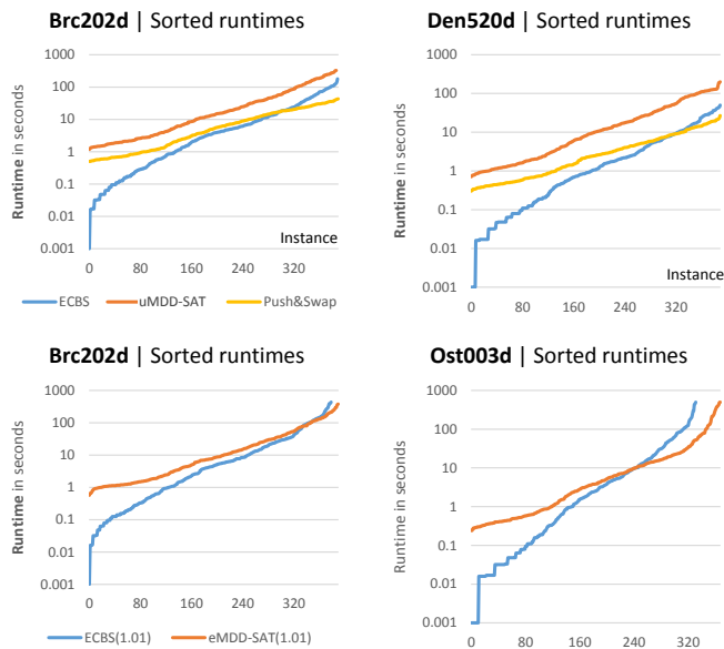
Figure 2: Runtimes of unbounded and bounded algorithms ( \epsilon = 0.01 ) on DAO maps brc202d , den520d , and ost003d .
